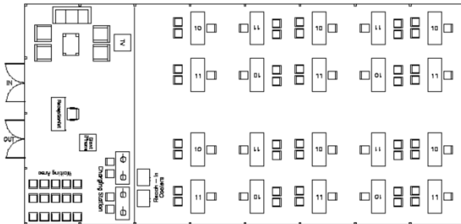
40' x 80' Structure
